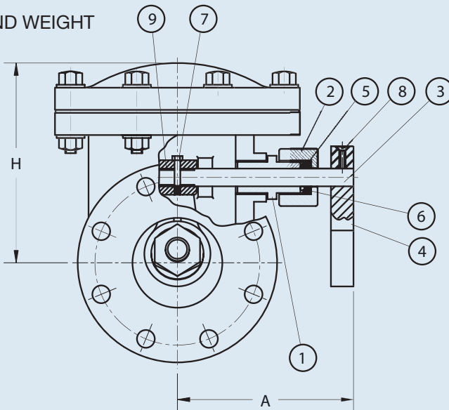
Dimensions (Sizes 3/4" – 8")
