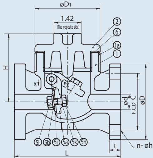
STANDARD MODEL 3/4"
