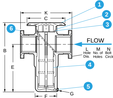
6" and 8" Design
